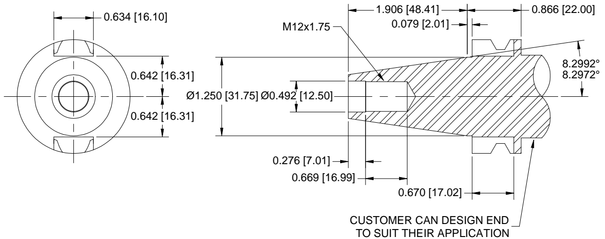
Figure 8. BT30 Toolholder Dimensions
