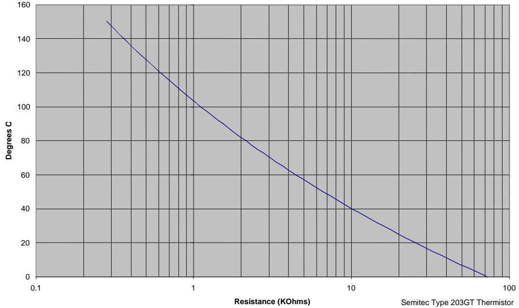
Figure 14. Thermistor Chart
