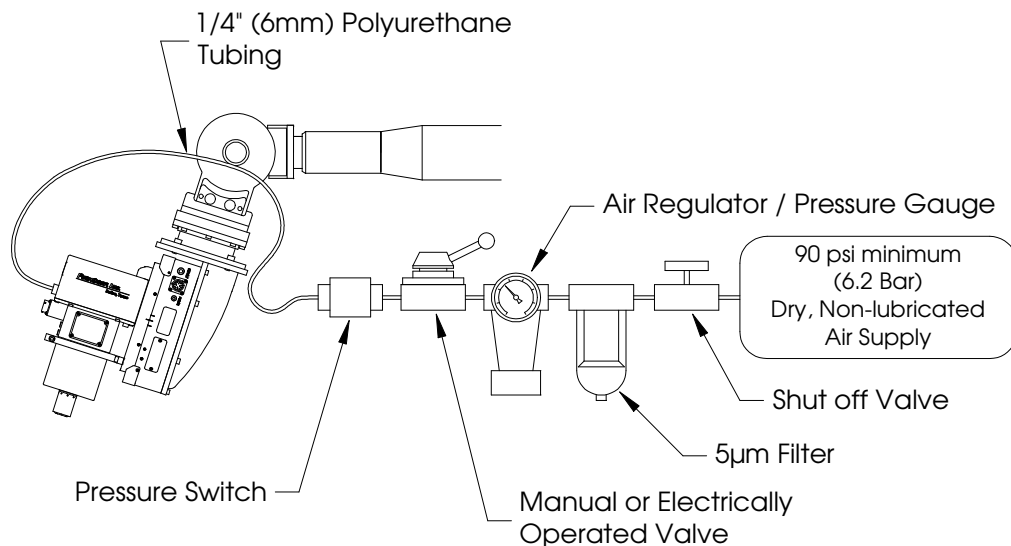
Figure 11. Pneumatic Connections
